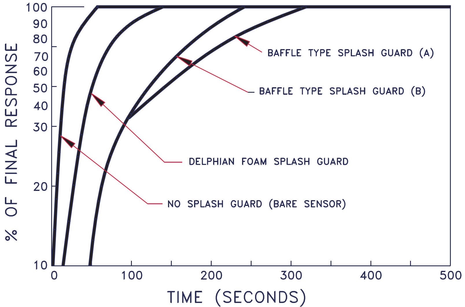
GAS SENSOR RESPONSE TIME WITH DIFFERENT SPLASH GUARDS 995181_A
